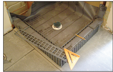
No. 543 Kirb-Perfect™ Shower Curb
